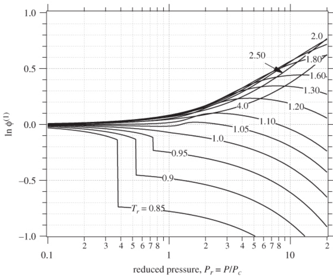
Figure 7-2: Generalized graph for (\ln \phi)^{(0)} and (\ln \phi)^{(1)} (extended range of pressures).
