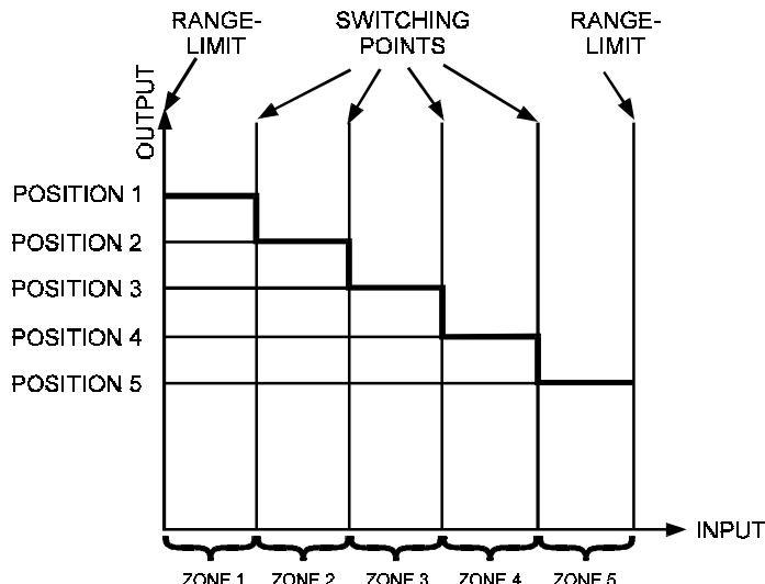
Figure 12 — Multi-position controller
