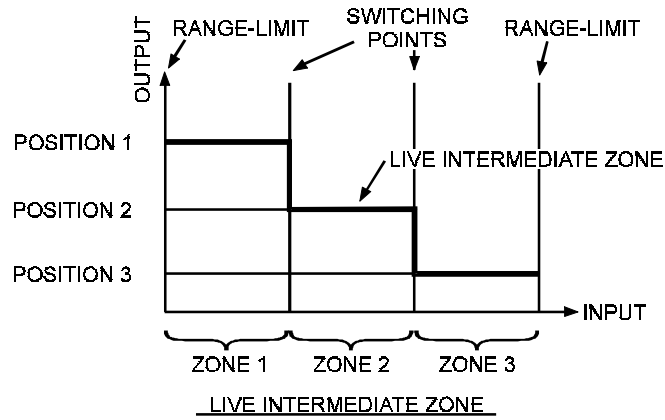
Figure 13 — Three-position controller
