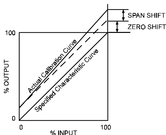
Figure 26 — Shift, span and zero
