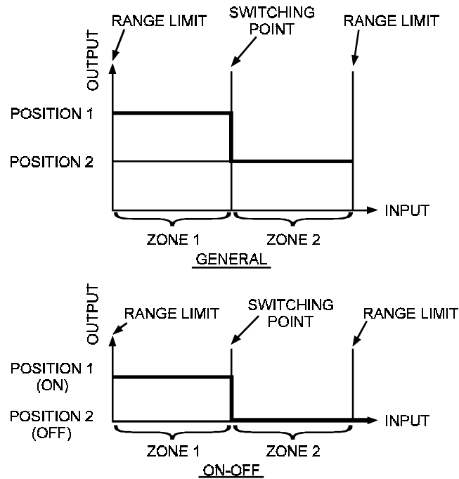
Figure 14 — Two-position controller
