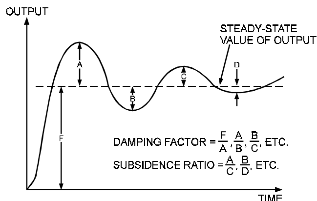
Figure 17 — Underdamped response of a system with second-order lag
