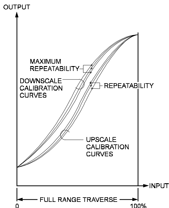
Figure 23 — Repeatability
