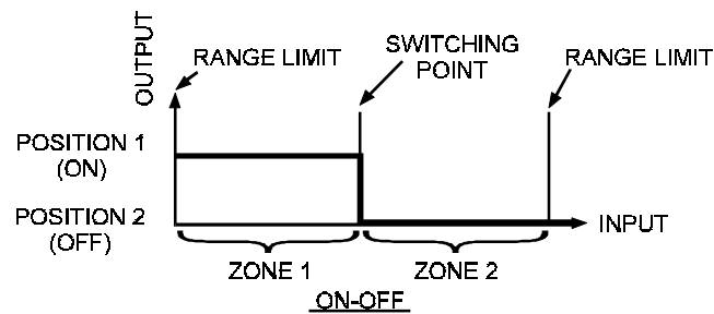
Figure 14 — Two-position controller
