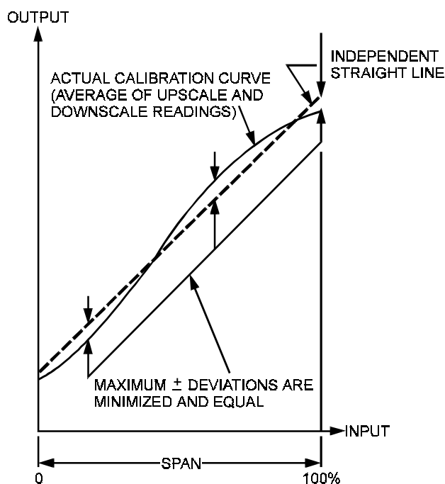
Figure 19 — Independent linearity
