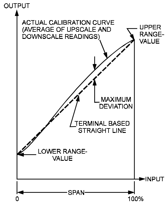
Figure 20 — Terminal-based linearity
