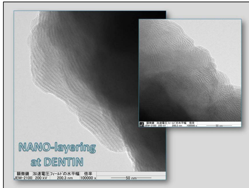
Fig. 5 – Even though hydroxyapatite in dentin differs chemically from pure hydroxyapatite and contains impurities, a similar nano-layering by 10-MDP could be observed by high-resolution TEM on dentin.
