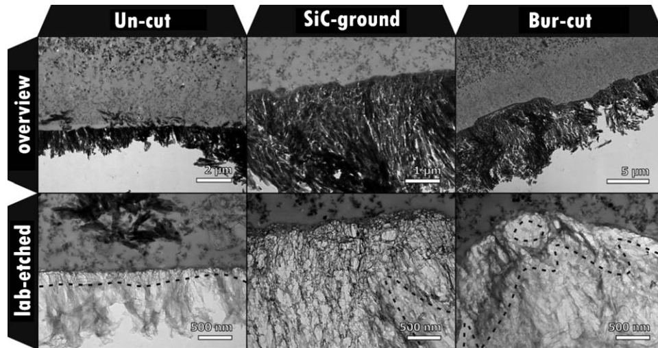
Fig. 9 – Transmission electron microscopy photomicrographs of Clearfil S 3 Bond (Kuraray) bonded to enamel that was prepared in three different manners: (1) solely pumiced (uncut, not prepared by bur), (2) ground by 600-grit SiC-paper, and (3) prepared by a coarse diamond bur. By demineralising (lab-etching) the sections [71], the actual depth of interaction could be evaluated more precisely (images at bottom).
