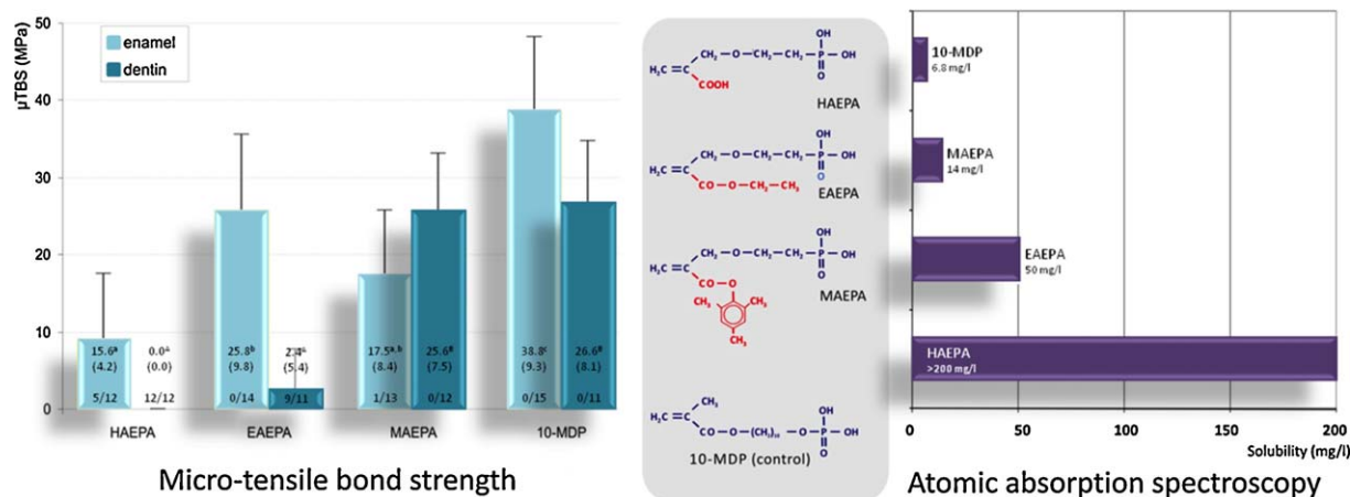
Fig. 8 – A study with experimental monomers confirmed that the chemical bonding capacity of functional monomers to calcium in hydroxyapatite co-determines the adhesive performance of adhesives. (left) The bond strength of three experimental phosphonate monomers synthesized by Vivadent-Ivoclar (Schaan, Liechtenstein: 2-[4-(dihydroxyphosphoryl)-2-oxabutyl]acrylate or HAEPA, ethyl 2-[4-(dihydroxyphosphoryl)-2-oxabutyl]acrylate or EAEPA, and 2,4,6 trimethylphenyl 2-[4-(dihydroxyphosphoryl)-2-oxabutyl]acrylate or MAEPA), was assessed and compared to that of 10-MDP as control. In terms of bonding effectiveness, MAEPA proved to be most effective and only at enamel, a significantly lower bond strength was measured as compared to 10-MDP. (right) Good bonding effectiveness corresponded to a low solubility of the respective Ca-salt.
