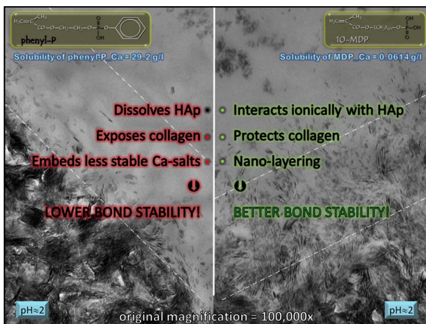
Fig. 7 – TEM images (non-demineralised sections) of the interaction of a phenyl-P-based adhesive (Clearfil Liner Bond 2, Kuraray) and a 10-MDP-based adhesive (Clearfil SE, Kuraray) with dentin. Due to the hydrolytic instability of the phenyl-P-Ca salt, this monomer rather demineralises dentin, whereas 10-MDP remains bonded to hydroxyapatite, resulting in much less demineralisation.
