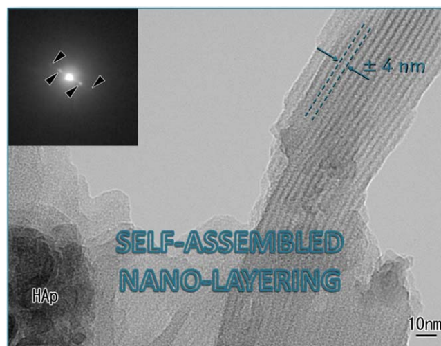
Fig. 4 – This high-resolution TEM image shows the formation of a self-assembled nano-layered structure on synthetic hydroxyapatite, that consists of 4-nm layers and is typically formed by 10-MDP. Each one of these layers consists of two 10-MDP monomers, that have assembled with their methacrylate groups directed toward each other and their phosphate groups directed away from each other.
