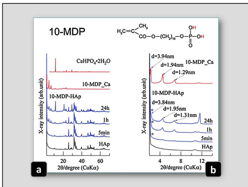
Fig. 6 – Powder XRD spectra showing the interaction of 10-MDP with synthetic hydroxyapatite (a: wide angle; b: low angle).
