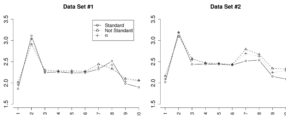
Fig. 5 Average O^I - Fe distances (Å), in docked poses
